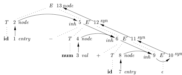
Dependency graph for a - 4 + c
